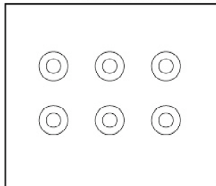
PD0954 DW WASHER (6), d5.5 x D11 x W0.2MM
