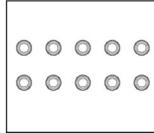
PD7659 BALL BEARING (10), d5 x D9 x W3MM
