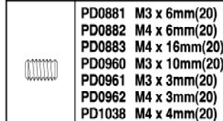
SET SCREW
